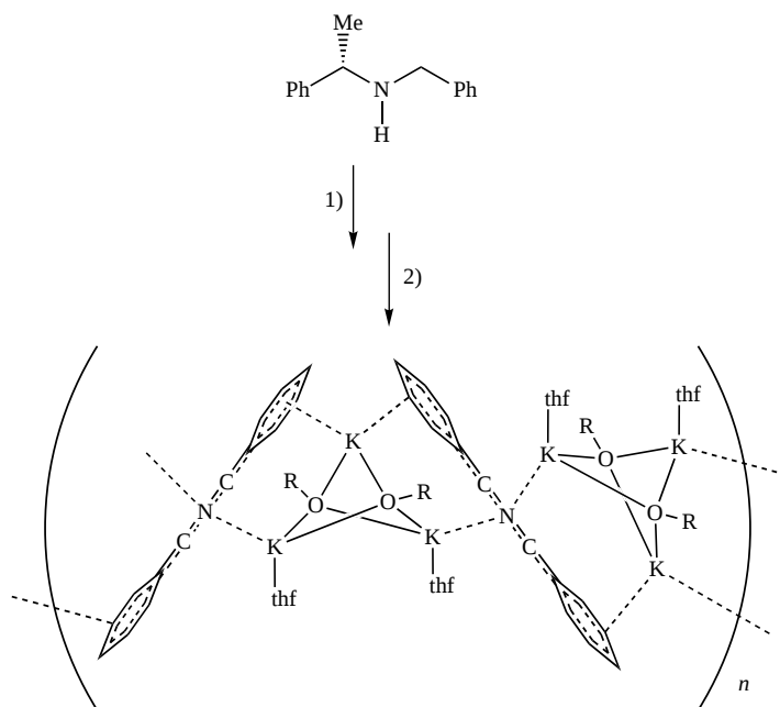
Scheme 1. Synthesis of 1 ; 1) 3 \text{tBuOK} , n\text{BuLi} , hexane, -78^\circ\text{C} ; 2) 2 tmen, THF ( -\text{hexane} ). \text{R} = \text{tBu} .
